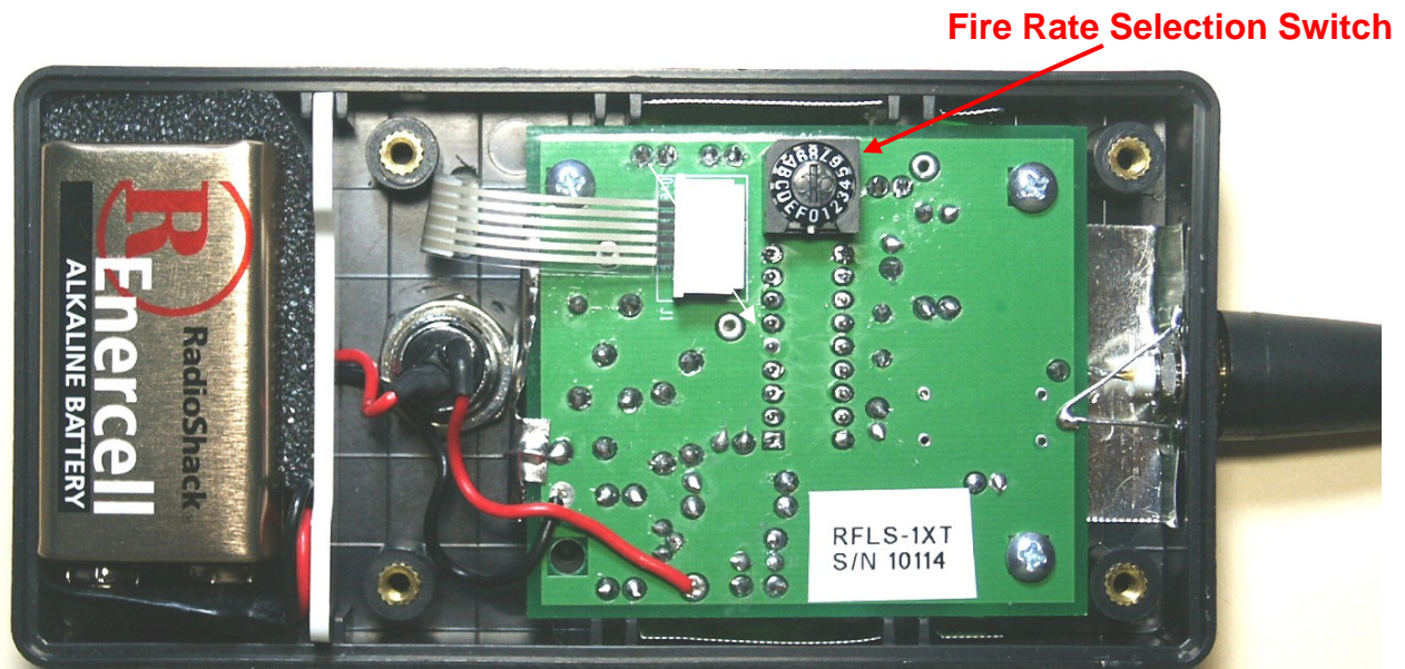
(Transmitter with rear cover removed)
